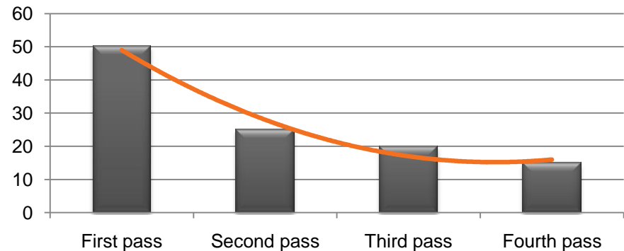
Compaction effect on waste layer
